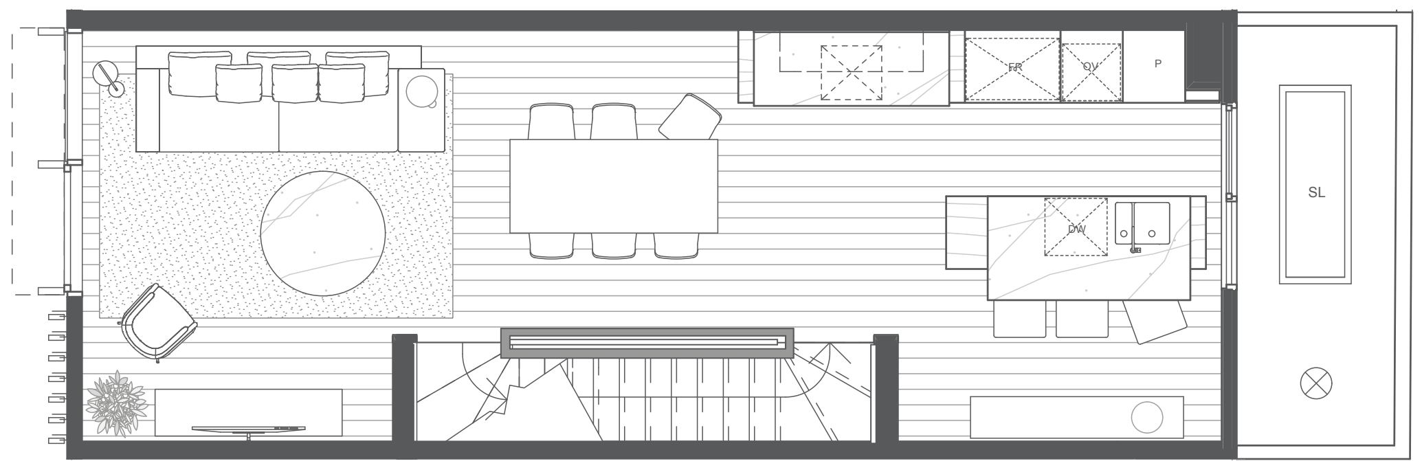
FIRST FLOOR
