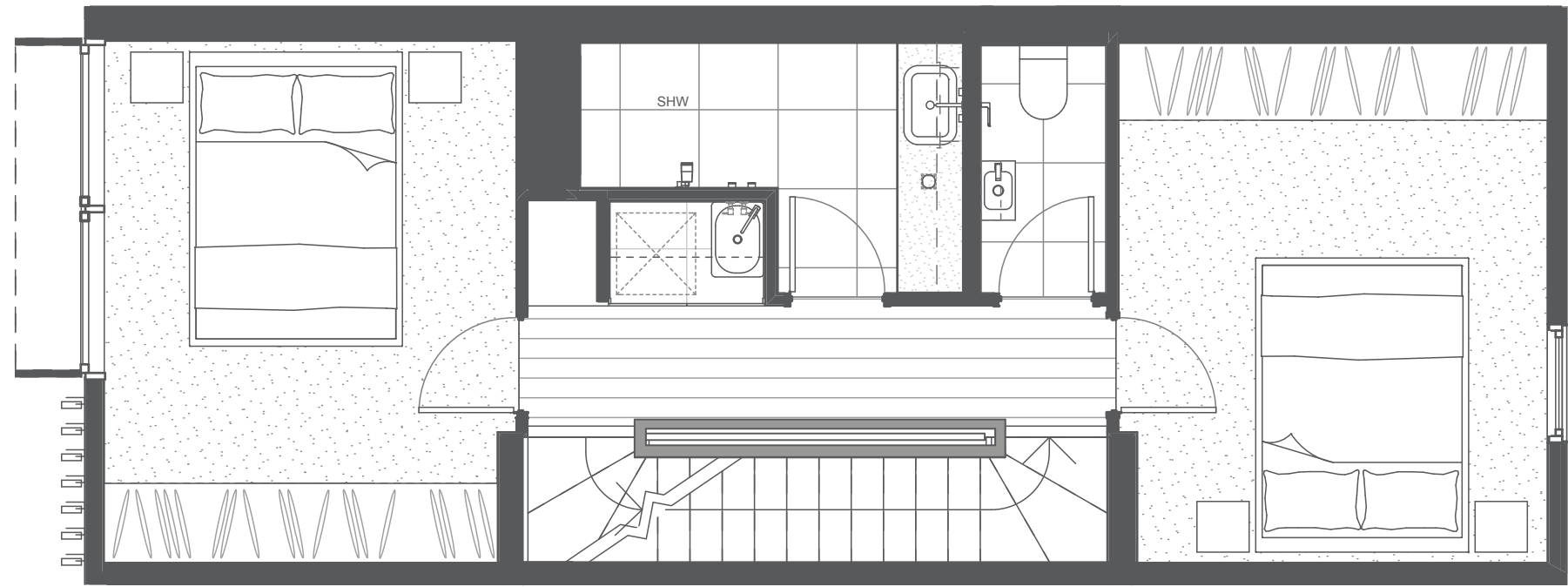
THIRD FLOOR
