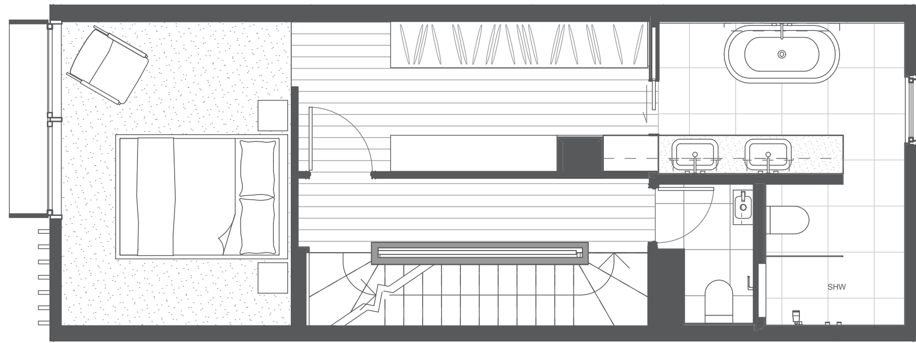
SECOND FLOOR
