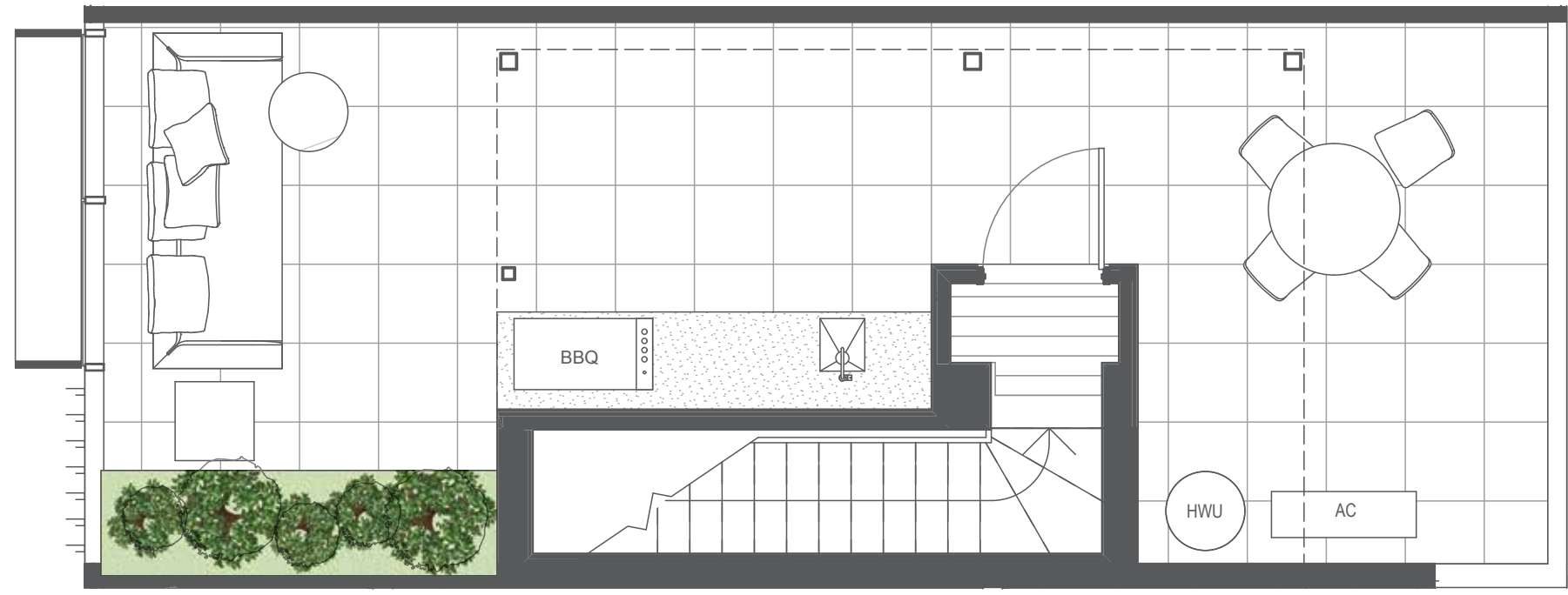
ROOFTOP
